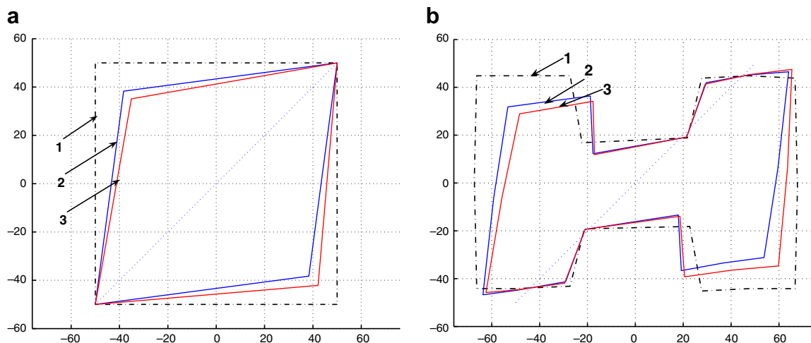
Fig. 5. Difference in the projection of two control polygons for the two camera models discussed, after rotating the camera 40° about a 45° axis on the target, passing through the target center. (1) Original contour, (2) weak-perspective projection, and (3) full-perspective projection. (a) Square shape (b) “H” shape.
