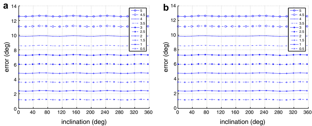
Fig. 11. Effects of introducing cyclorotation in the camera motion. Each line is the recovery error after a camera rotation about an axis passing through the target, and whose orientation varies from 0° to 360° in the plane, and from 0.5° to 5° out of the plane (increasing the amount of cyclorotation). (a) Square shape (b) “H” shape.
