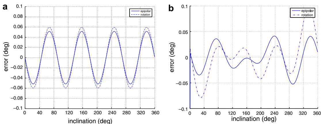
Fig. 6. Error in the recovery after a camera rotation of 40^\circ about an axis passing through the target centroid and whose orientation varies from 0^\circ to 360^\circ . The continuous line shows the error in the recovery of the epipolar direction, while the dotted one indicates the error in the recovery of the orientation of the rotation axis. (a) Square shape (b) "H" shape.
