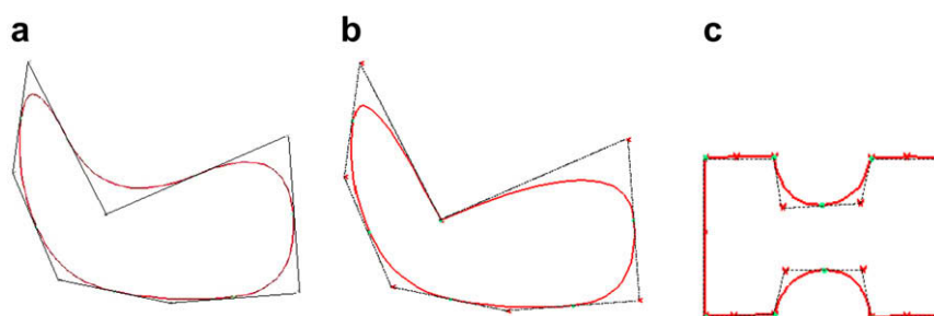
Fig. 4. Representing contours using B-splines: (a) and (b) show that different contours can be modelled with the same control polygon but different knot multiplicities, while (c) displays the modelling of the H-shaped contour used in the experiments. (a) 7 Control points (b) 7 control points and 1 double knot (c) 18 control points and 8 double knots.
