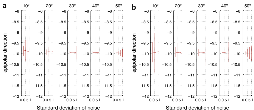
Fig. 9. Error in the recovery of the epipolar direction for a rotation axis of 45° when the rotations through this axis range from 10° to 50° and depth relief is introduced adding Gaussian noise with \sigma = 0.25, 0.5, 0.75 and 1 in the direction perpendicular to the image plane. (a) Square shape (b) "H" shape
