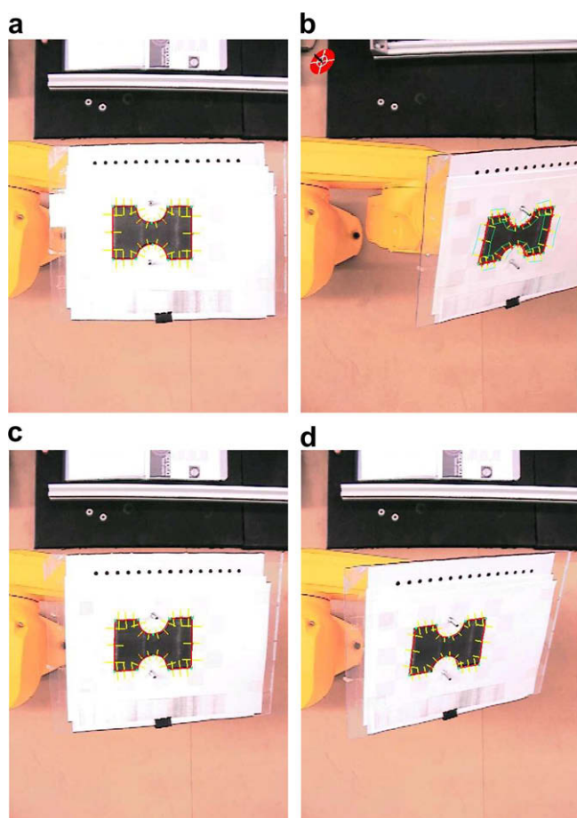
Fig. 15. Experiments with real images further relaxing weak-perspective conditions. The first sequence, entailing an uncentered target, starts at (a) and ends at (b). The next sequence departing from a non-frontoparallel target position starts at (c) and ends at (d). The last sequence, testing also non-frontoparallel initialization, starts at (d) and ends at (a). (a) Initial, (b) lateral translation and 40° (c) 20° (d) 40°.
