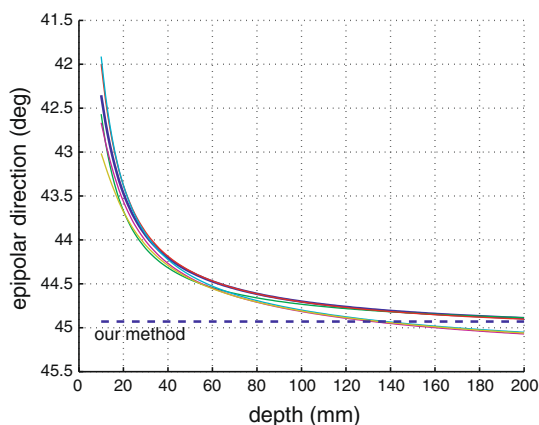
Fig. 13. Epipolar direction computed with the GS algorithm in the case of 2, 4, ..., 12 out-of-plane points (a curve for each number) placed at increasing depths (in abscissae) above the H-shaped contour. Notice that the relevant factor is not the number of points, but the depth at which they are placed.
