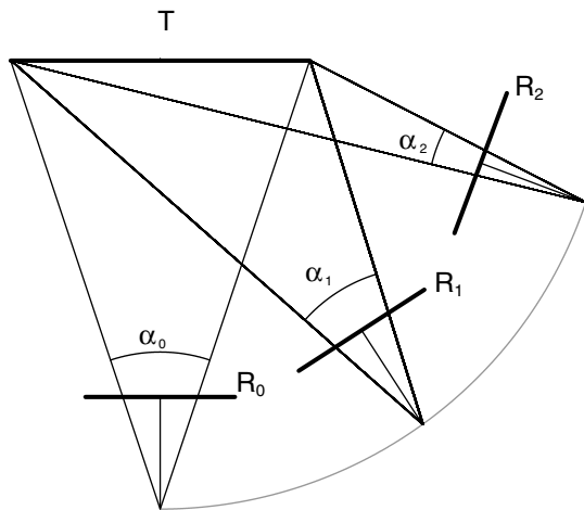
Fig. 8. Starting with a frontoparallel target T , a first view R_0 is taken and then two other views R_1 and R_2 are taken; R_2 after a larger amount of rotation than R_1 . The maximum angle \alpha_i between the rays of the target projection decreases (and, thus, the projection becomes closer to a parallel projection) as the amount of rotation increases.
