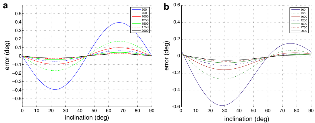
Fig. 7. Error in the recovery of the epipolar direction when the distance from the camera to the target varies from 500 to 2000 mm. The plot shows results for a camera rotation of 40° about an axis on the target with inclinations ranging from 0° to 90°. (a) Square shape (b) "H" shape.
