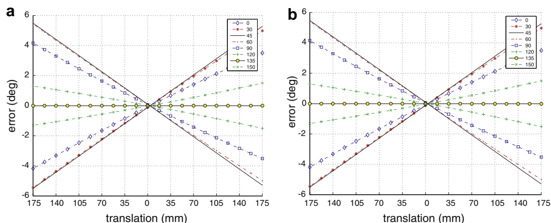
Fig. 10. Error in the recovery of the epipolar direction for a fixed rotation of 40^\circ about an axis inclined 45^\circ on the target plane and an initial distance of 5 m, when lateral translations of the camera along the several directions listed in the insert are performed. (a) Square shape (b) “H” shape.
