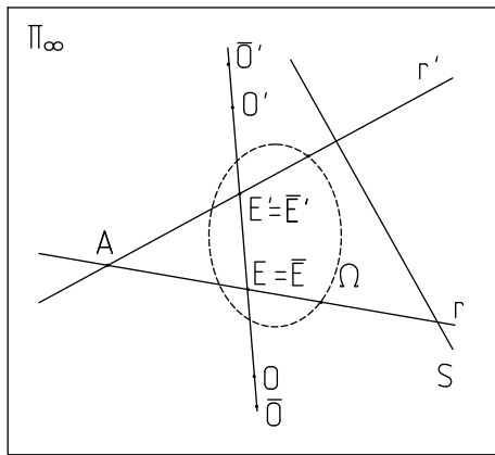
Fig. B.2. Geometry on the plane at infinity of two affine cameras under the hypothesis of Theorem 4. The notations are clear from the text.
