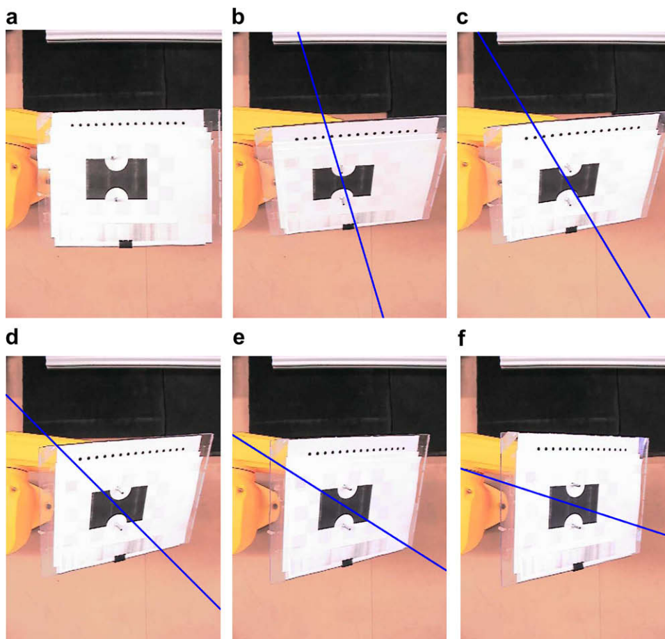
Fig. 14. The first experiment with real images entails pairs of views consisting of the initial one plus each of the other five, corresponding to camera rotations of 40^\circ about an axis on the target with inclinations sampled at intervals of 15^\circ . The computed epipolar direction is displayed as a line passing through the target center. (a) Initial (b) 15^\circ (c) 30^\circ (d) 45^\circ (e) 60^\circ (f) 75^\circ .
